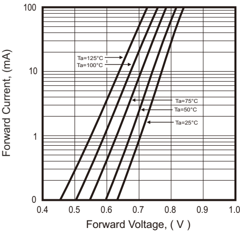
Fig.4 - Forward Characteristic
